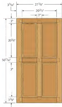
BACK PANEL
